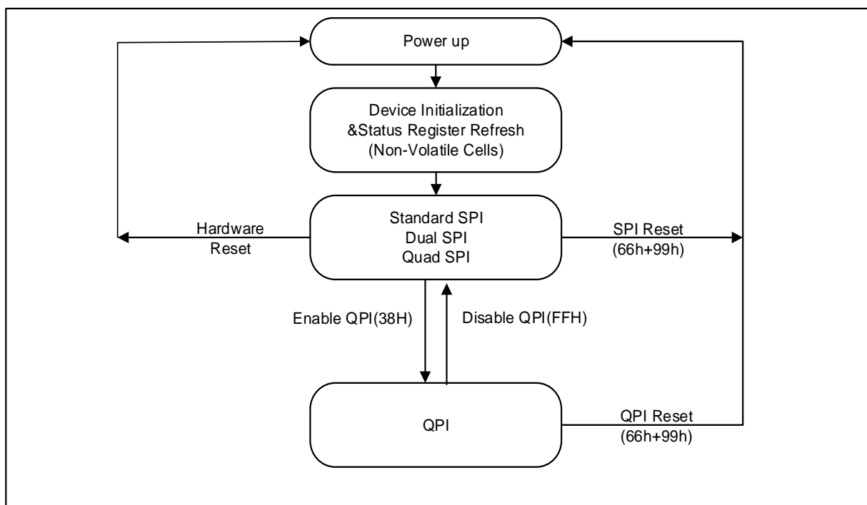
Figure 3. XM25QW32C Serial Flash Memory Operation Diagram
