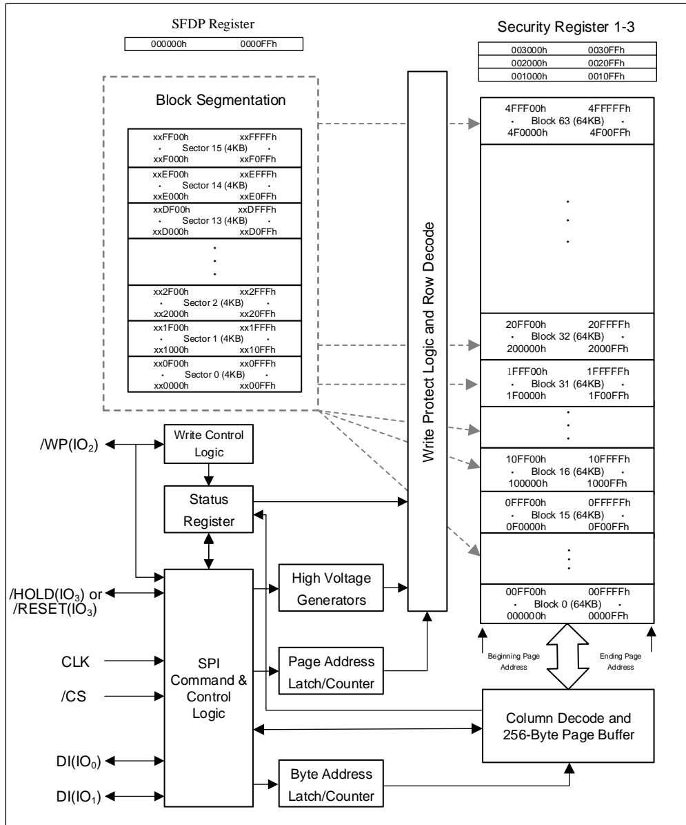
Figure 1. XM25QW32C Serial Flash Memory Block Diagram
