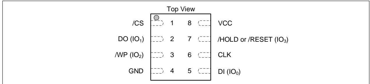
Figure 2b. 8-pad WSON 5x6-mm (Package Code W)/8-pad USON 4x3-mm (Package Code U2)
