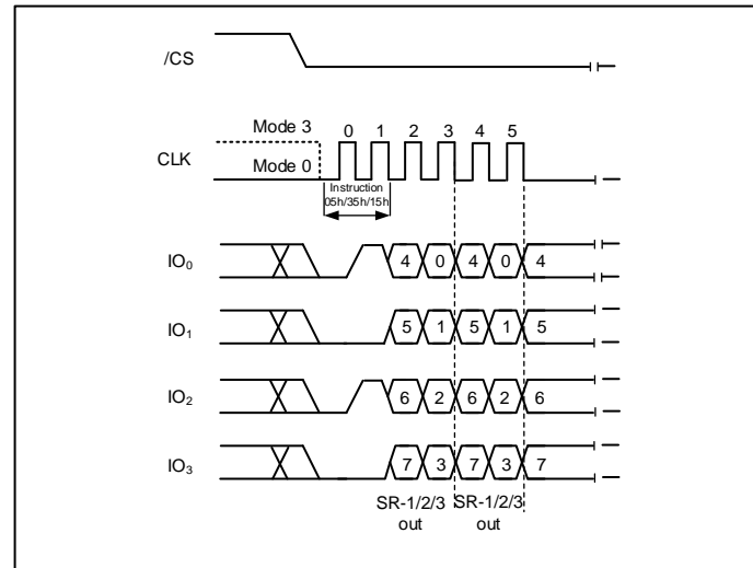
Figure 8b. Read Status Register Instruction (QPI Mode)
