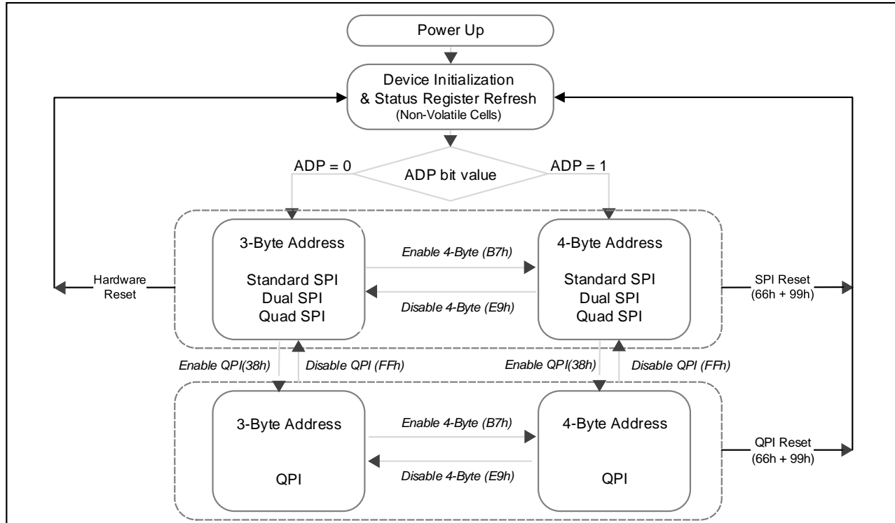
Figure 3. XM25QU512C Serial Flash Memory Operation Diagram
