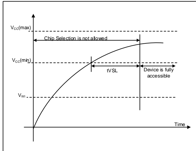
Figure 59a Power-up Timing and Voltage Levels
