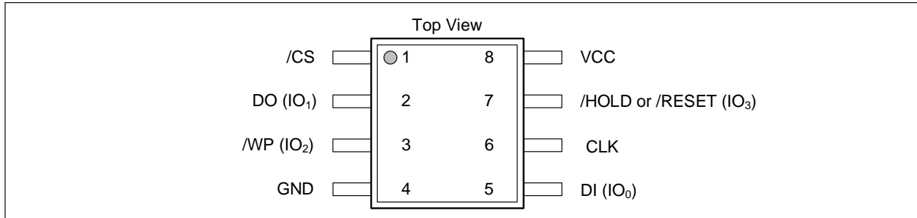
Figure 2b. 8-pin WSON 8L (Package Code X)
