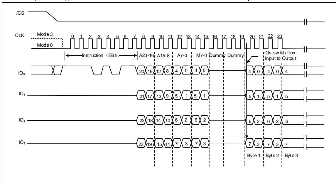
Figure 24a. Fast Read Quad I/O (Initial instruction or previous M5-4≠10, SPI Mode) 32-Bit Address is required when the device is operating in 4-Byte Address Mode
