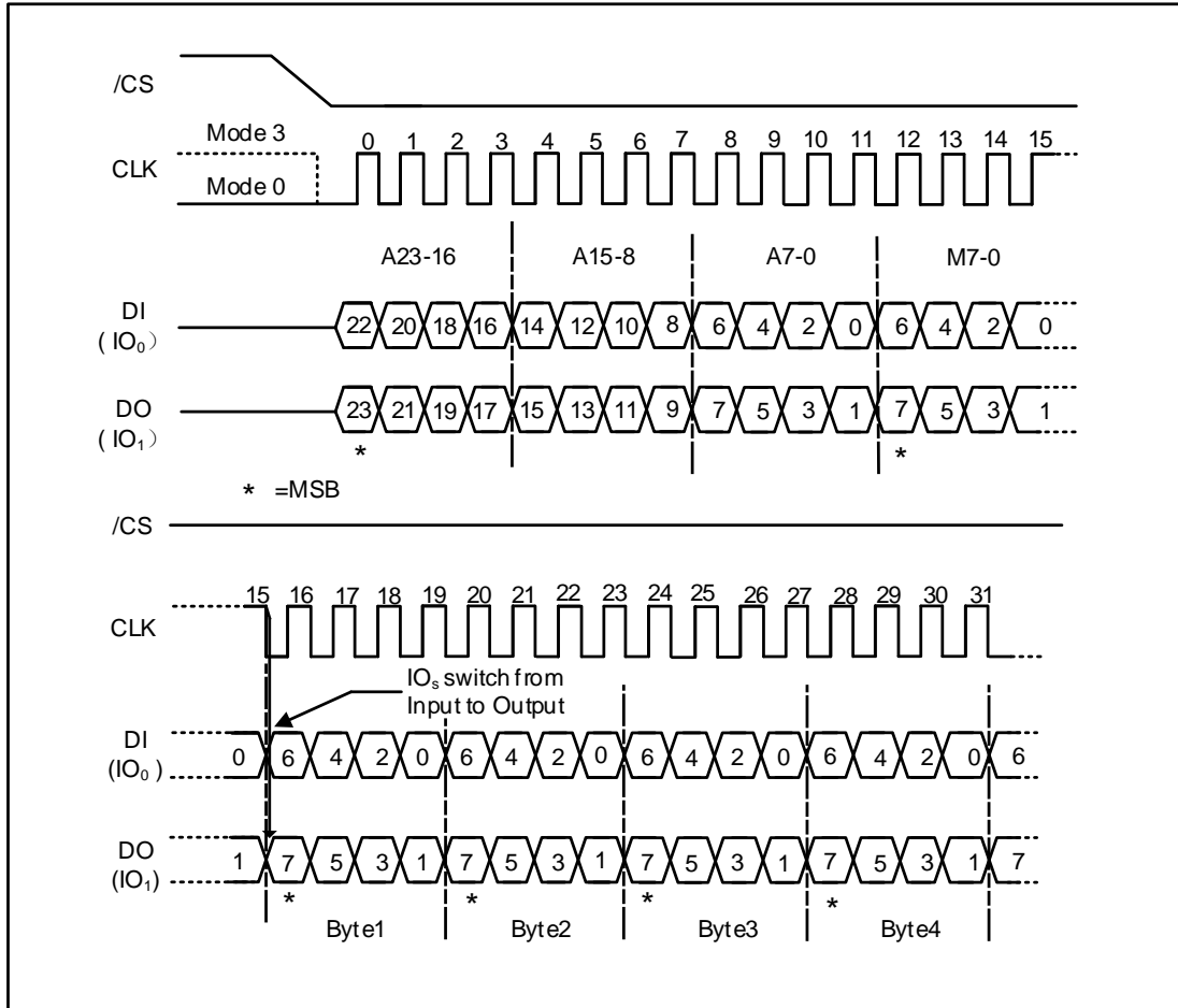
Figure 22b. Fast Read Dual I/O (Previous instruction set M5-4=10, SPI Mode only)
