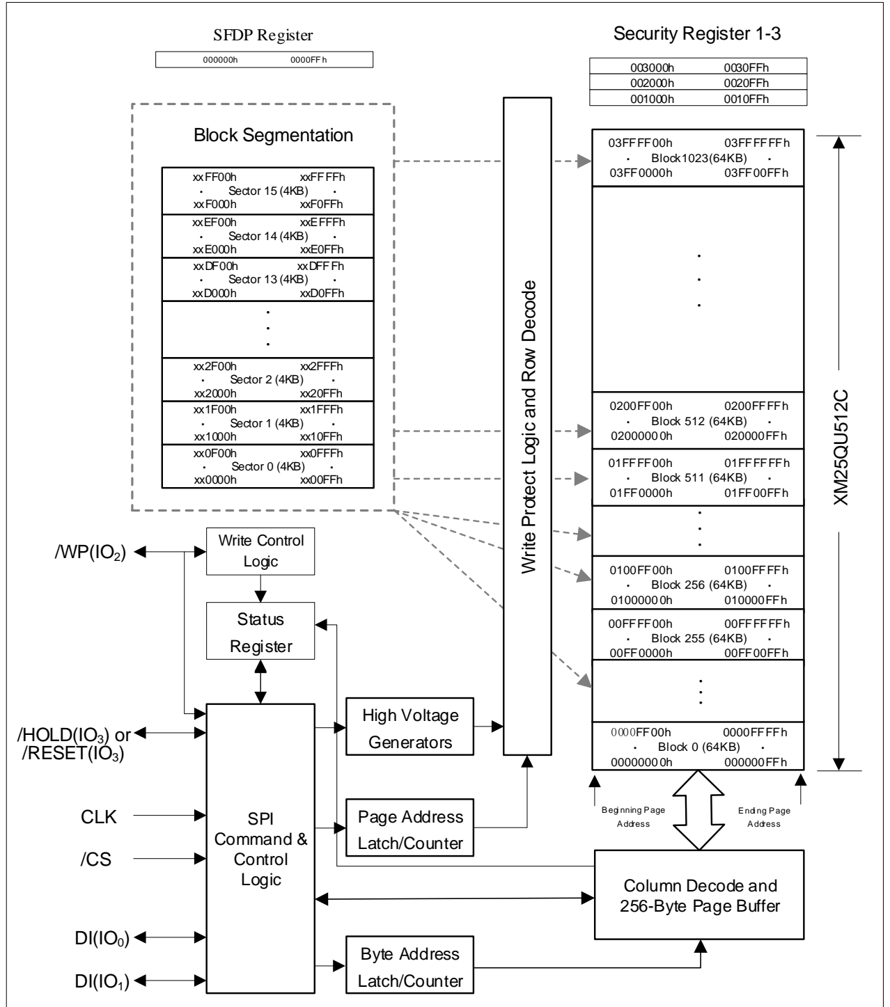
Figure 1. XM25QU512C Serial Flash Memory Block Diagram
