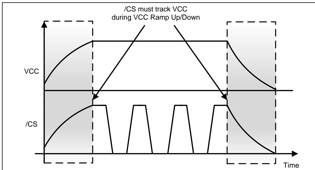
Figure 59b. Power-up, Power-Down Requirement
