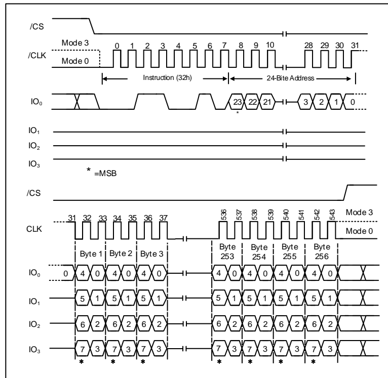
Figure 30. Quad Input Page Program Instruction (SPI Mode only)
