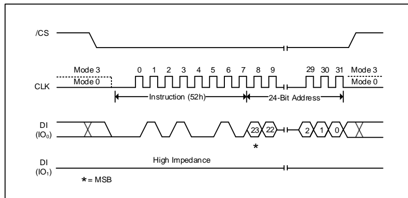
Figure 35a. 32KB Block Erase Instruction (SPI Mode) 32-Bit Address is required when the device is operating in 4-Byte Address Mode
