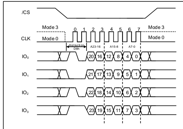
Figure 36b. 64KB Block Erase Instruction (QPI Mode)
