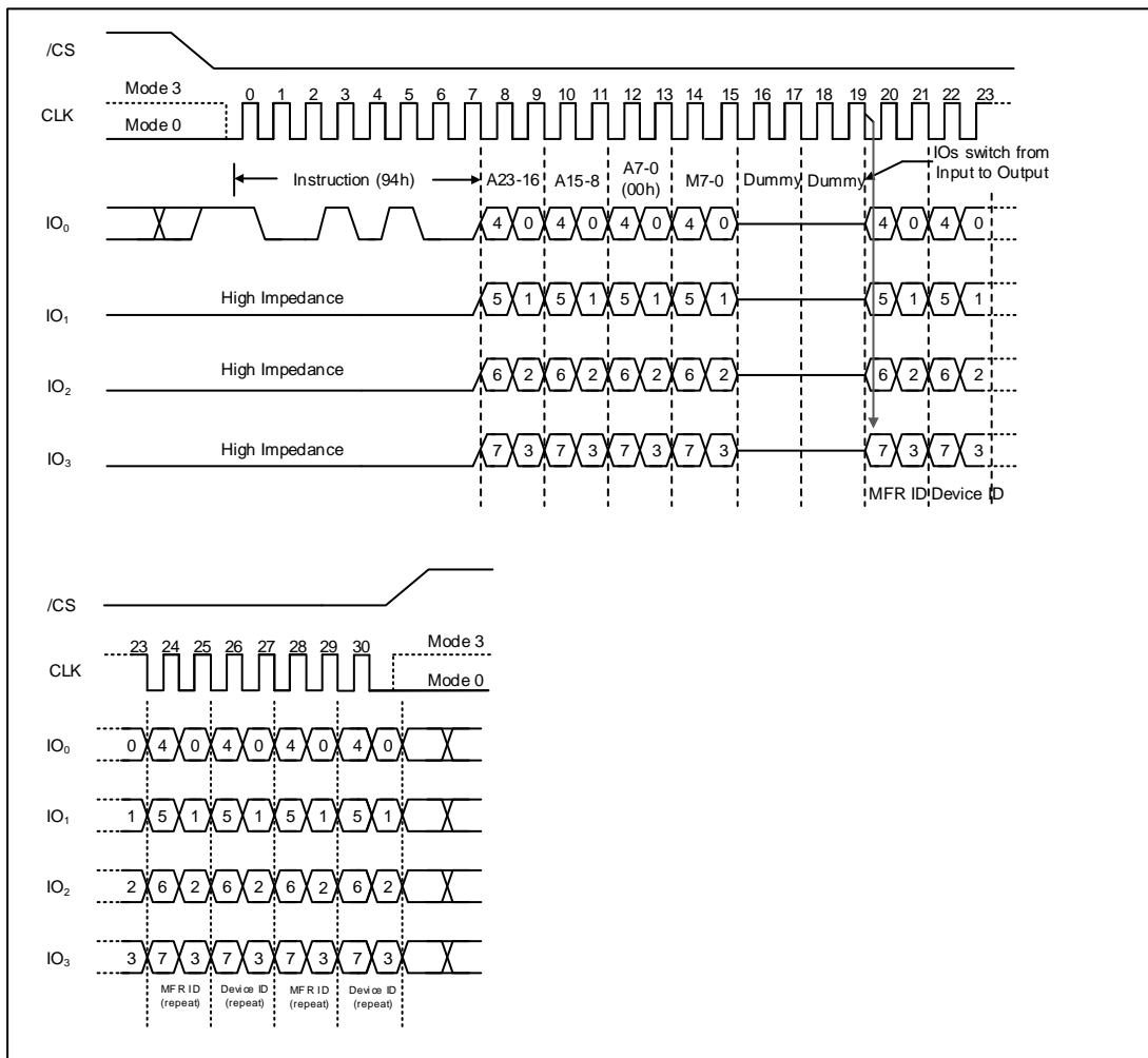
Figure 45. Read Manufacturer / Device ID Quad I/O Instruction (SPI Mode only)
