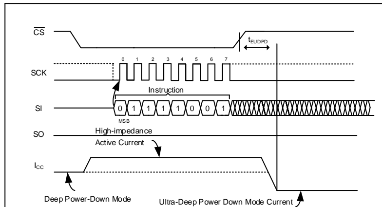
Figure 57. Ultra-Deep Power-Down
