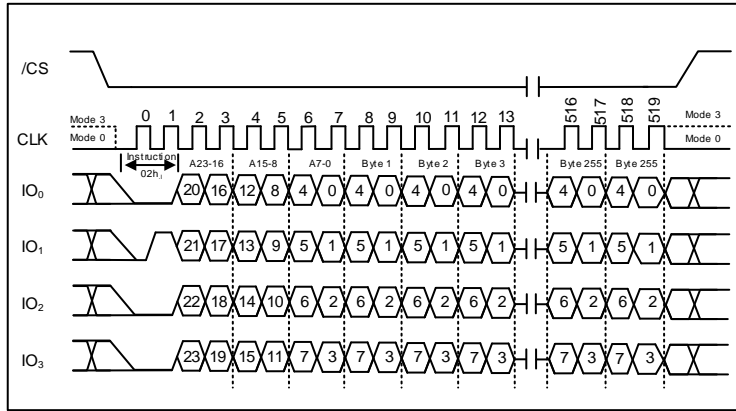
Figure 28b. Page Program Instruction (QPI Mode)
