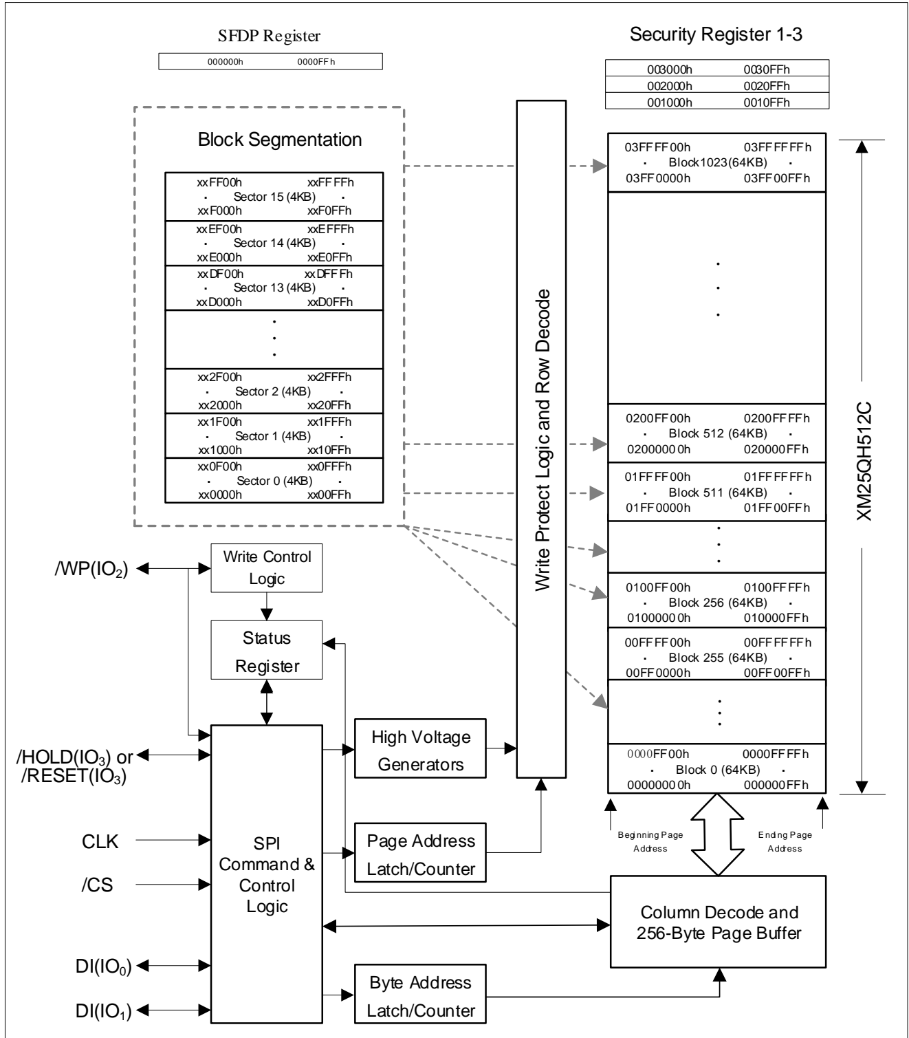
Figure 1. XM25QH512C Serial Flash Memory Block Diagram
