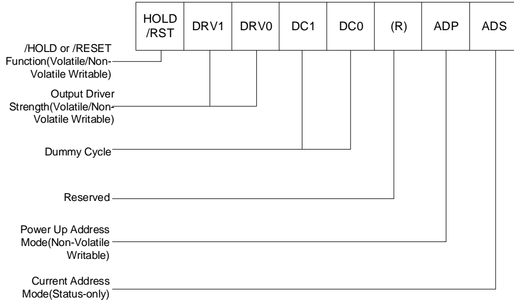
Figure 4c. Status Register-3
