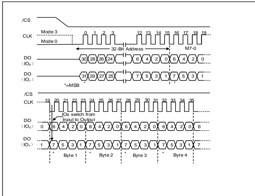
Figure 23a. Fast Read Dual I/O with 4-Byte Address Instruction. (Previous instruction set M5-4 ≠ 10, SPI Mode only)
