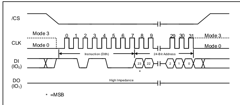
Figure 36a. 64KB Block Erase Instruction (SPI Mode)
