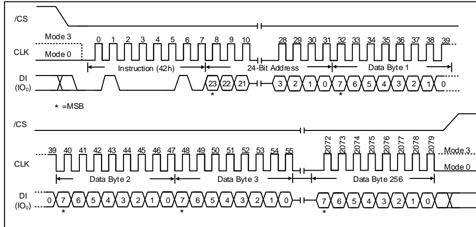
Figure 50. Program Security Registers Instruction (SPI Mode only)
