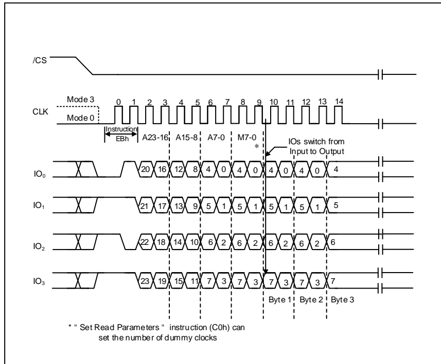
Figure 24c. Fast Read Quad I/O (Initial instruction or previous M5-4≠10, QPI Mode) 32-Bit Address is required when the device is operating in 4-Byte Address Mode
