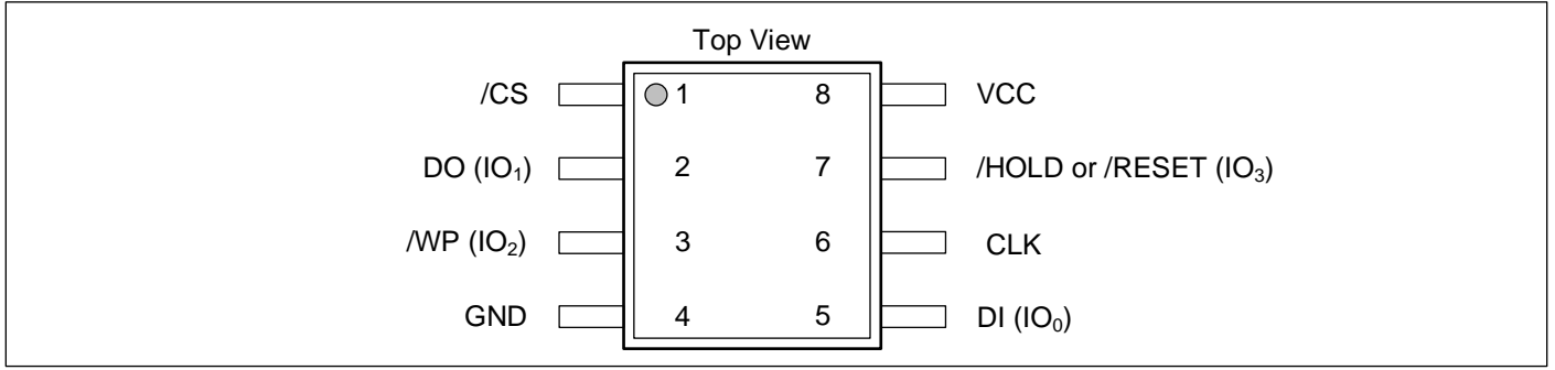
Figure 2b. 8-pin WSON 8L (Package Code X)
