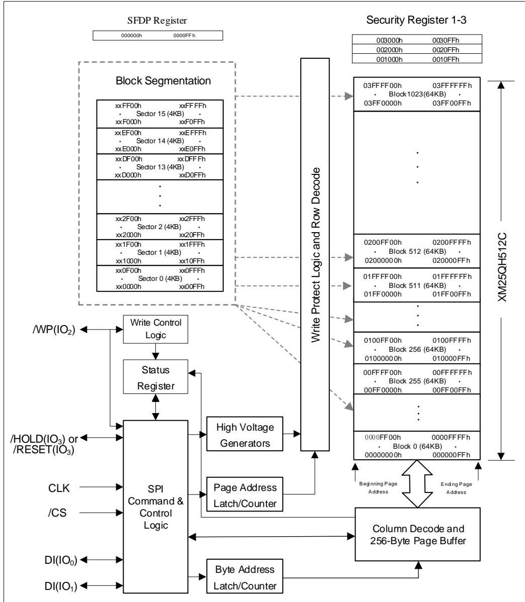
Figure 1. XM25QW512C Serial Flash Memory Block Diagram
